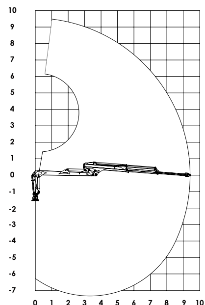
Reach diagram
