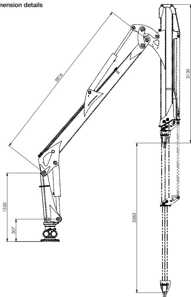
Dimension details
