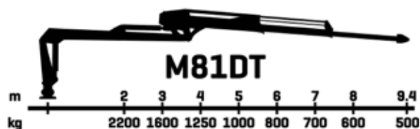
Lift capacity
